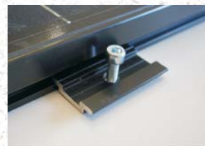
Aluminium Clips
